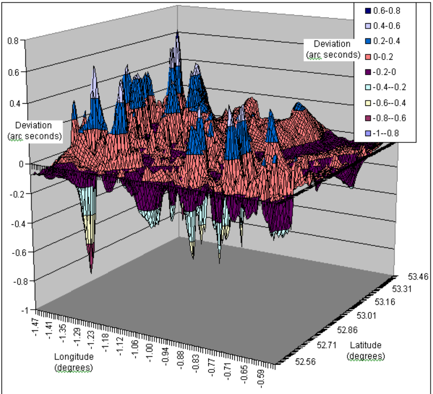
Nottingham Block east-west topographic-isostatic deviation
