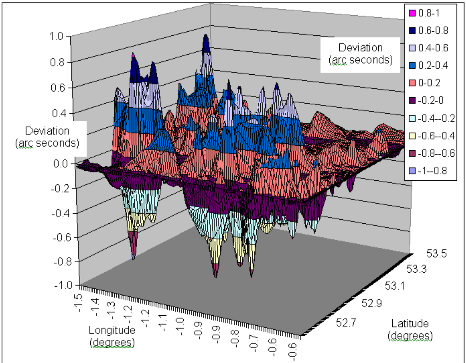
Nottingham Block north-south topographic-isostatic deviation
